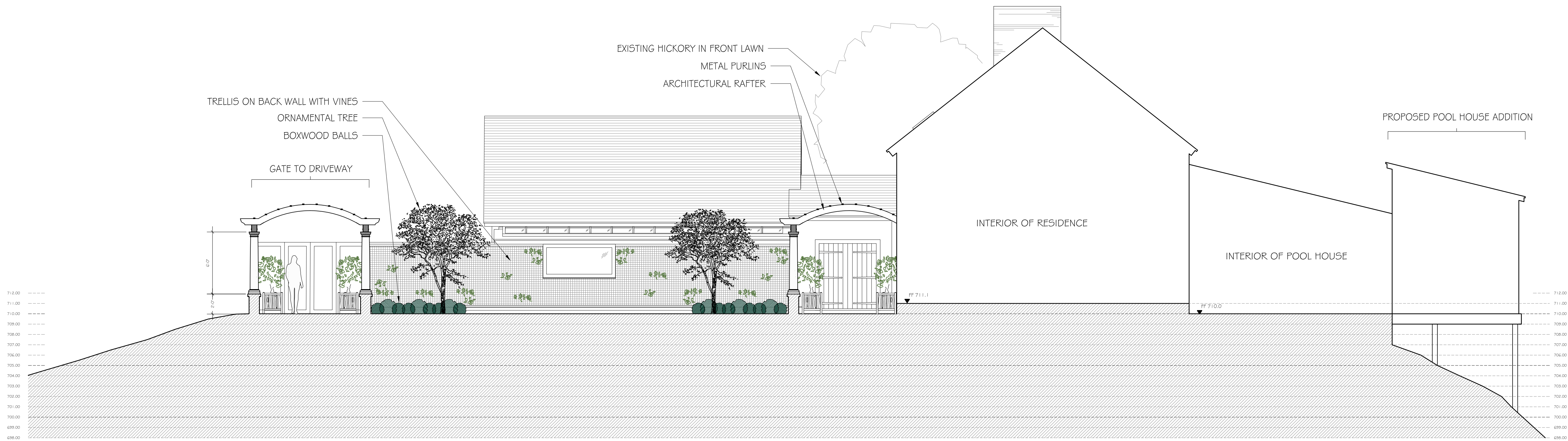
5 SECTION E-E' 3/16" = 1'-0"
